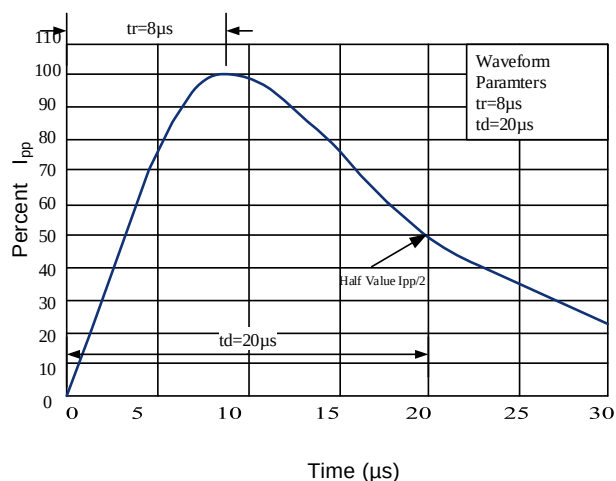
Figure 5: Pulse Waveform
